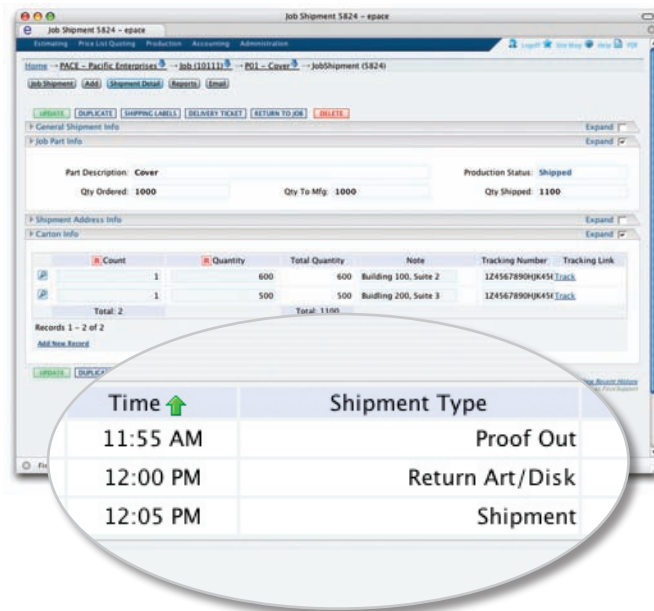
The Job Shipment Detail Screen
